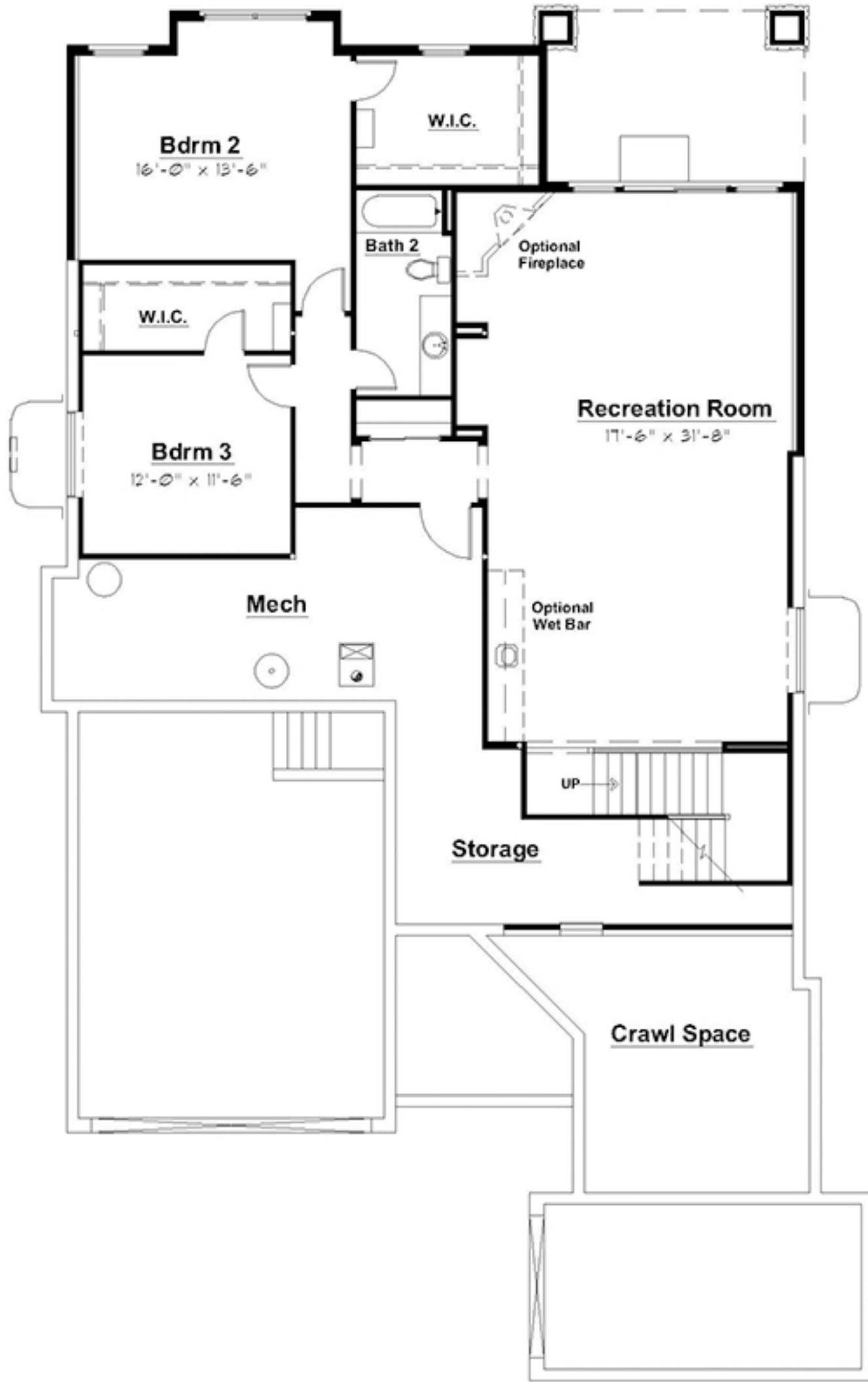
FINISHED BASEMENT PLAN STANDARD
